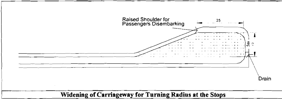
Widening of Carriageway for Turning Radius at the Stops
