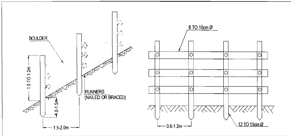
Figure 9.3: Layout and Design Specification for Bally Benching
