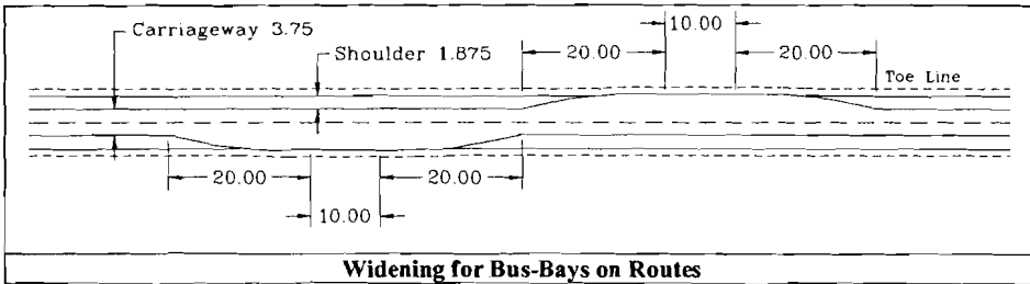
Widening for Bus-Bays on Routes
