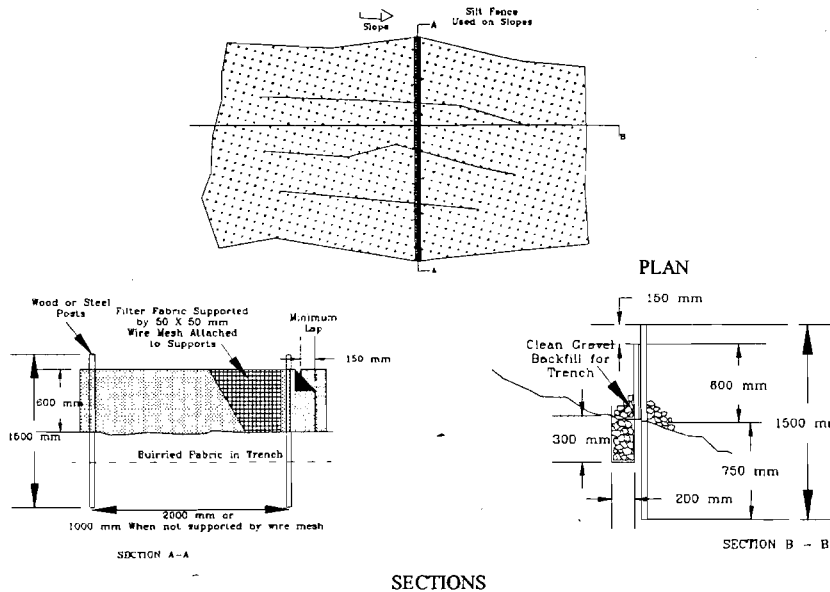
Figure 9.5 Cross-section of Silt Fencing
