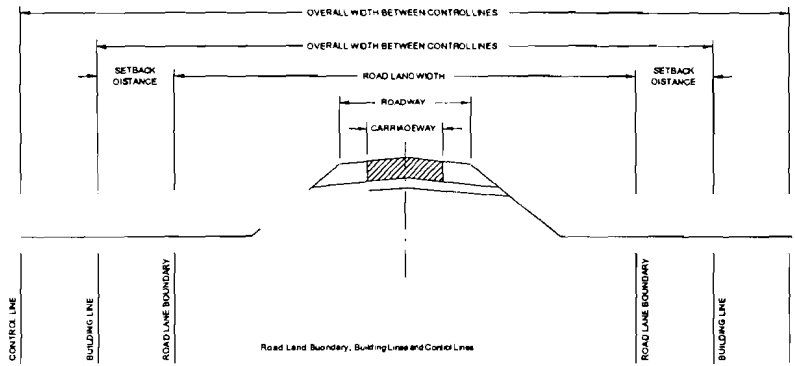
Typical Cross sections of PMGSY roads
