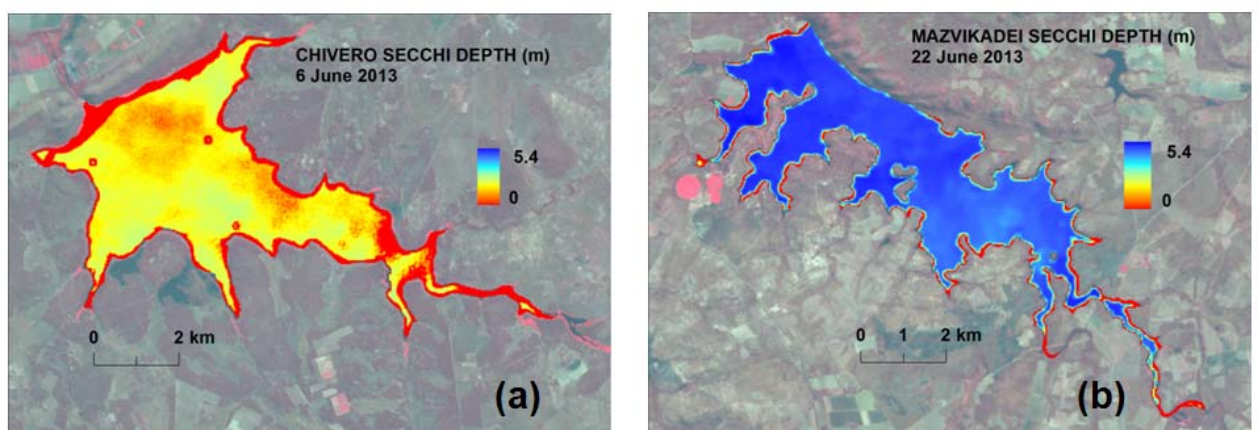
Figure 15: Maps of Secchi depth concentration in Lake Chivero (a) and Mazvikadei (b) reservoirs predicted from linear regression models developed from Landsat 8 satellite data calibrated with ground-measured data. The maps are overlaid on top of a false colour composite of consisting of Landsat bands, 5, 4 and 2.
