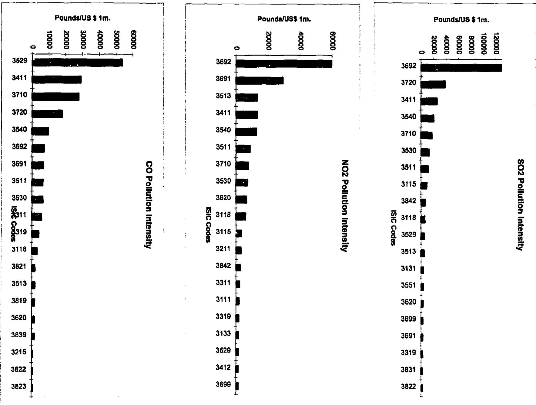
Figure 5.3 - Air Pollution Intensity for Selected Sectors
