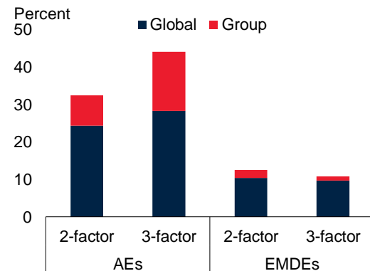
Figure A.3 Robustness of dynamic factor estimation to dynamic factor specification
