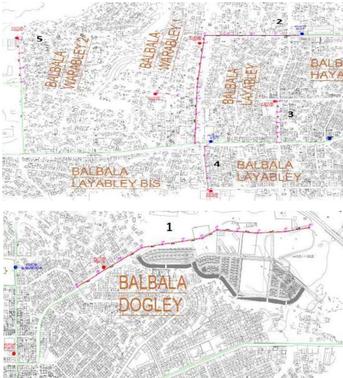
Figure 2.6. Routing of MV Lines in Balbala North
