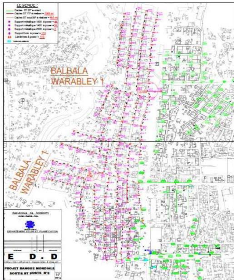
Figure 2.7. Localization of LV Lines in Warabley 1 Neighborhood in Balbala North
