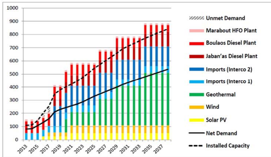
Figure 1. Djibouti’s Supply-Demand Balance 2017-2037
