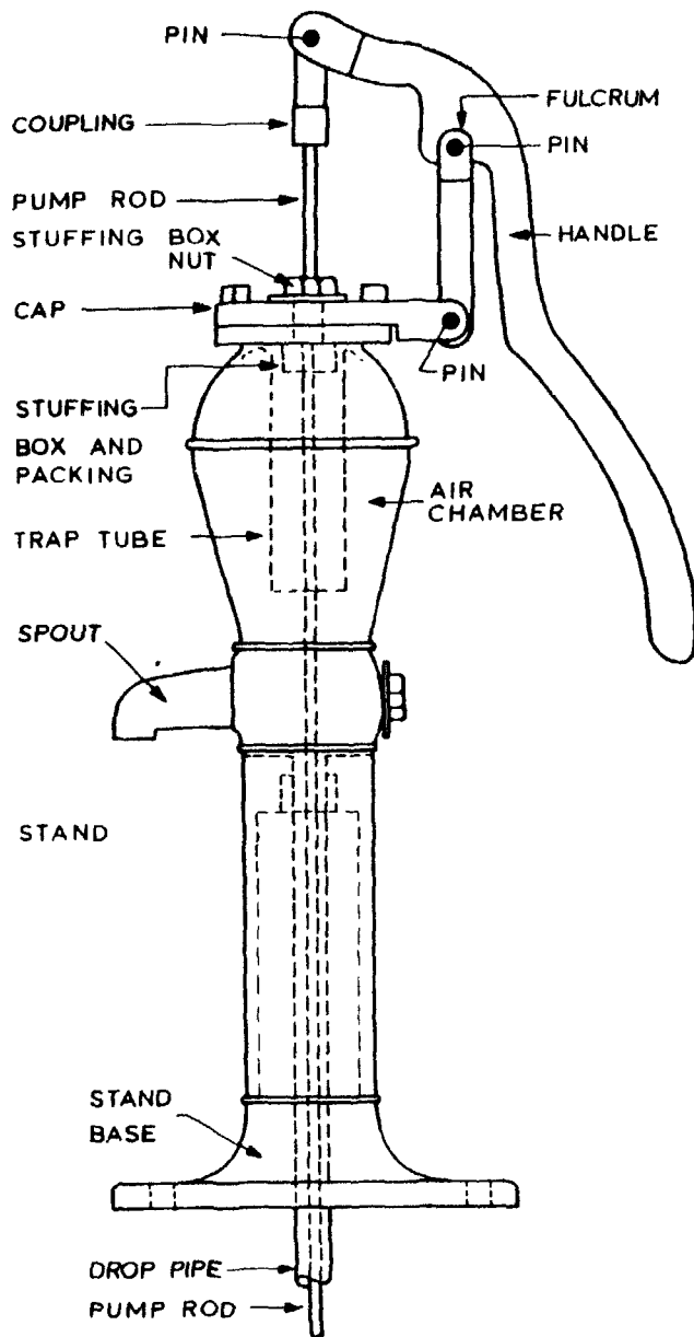
HAND PUMP WITH STUFFING BOX AND GUIDED PUMP ROD SUITABLE FOR USE AS A FORCE PUMP
