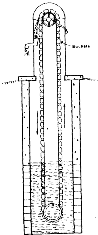
BUCKET PUMP
