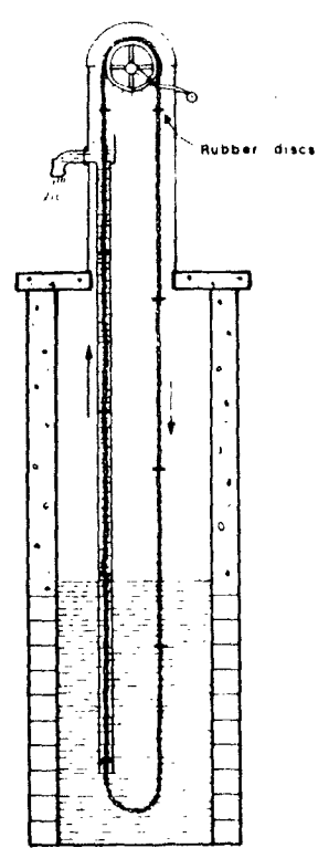
CHAIN PUMP
