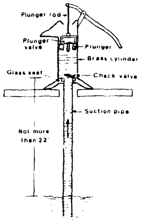
TYPICAL SHALLOW WELL LIFT PUMP
