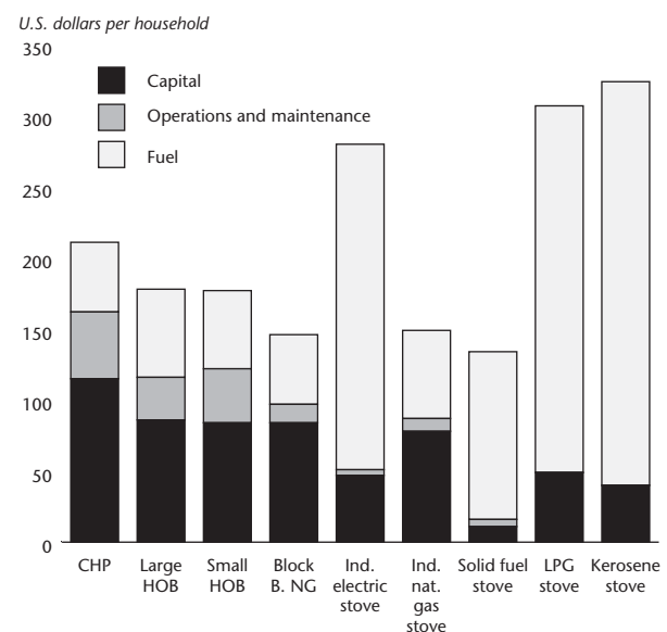
Figure 4-2 Annual costs of different heating options for full heat service in Yerevan, Armenia
