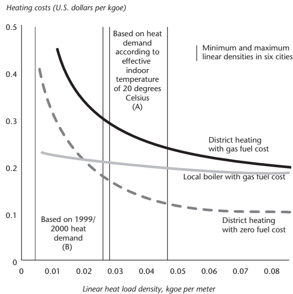
Figure 4-1 Costs of different heat supply options in Moldova
