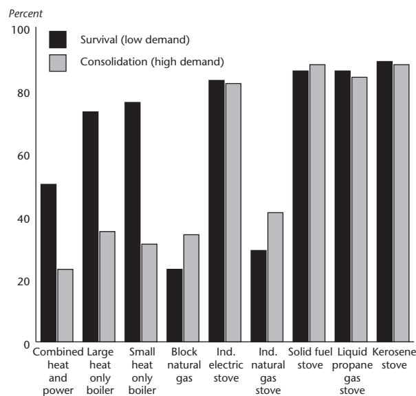
Figure 4-4 Fuel costs as share of total heat costs for different heat supply options and demand levels, Yerevan, Armenia
